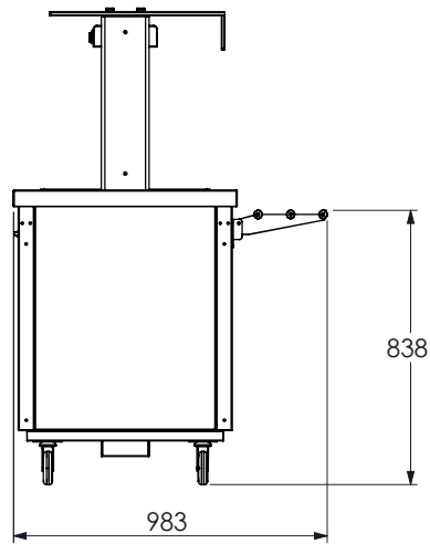
757 With tray slide in the down position
